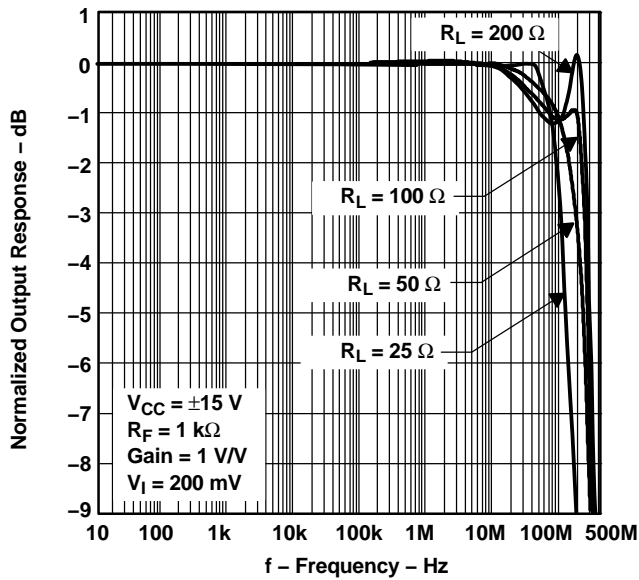
Figure 29. Normalized Output Response vs Frequency
