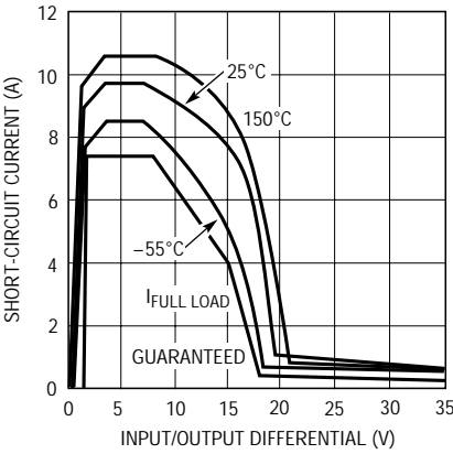
LT1083 Short-Circuit Current
