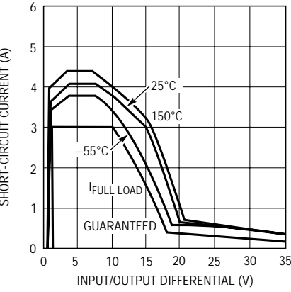
LT1085 Short-Circuit Current
