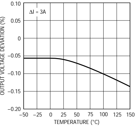
LT1085 Load Regulation
