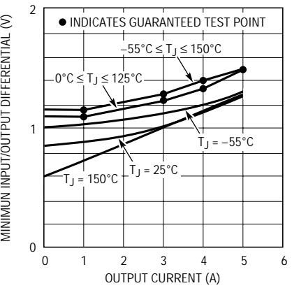
LT1084 Dropout Voltage
