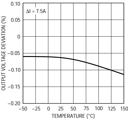
LT1083 Load Regulation
