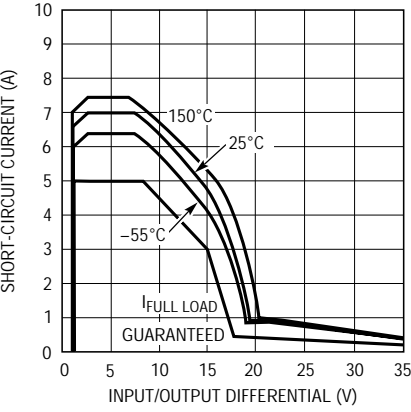
LT1084 Short-Circuit Current
