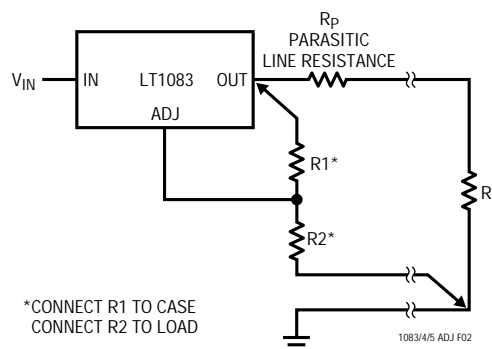
Figure 2. Connections for Best Load Regulation
