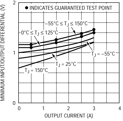
LT1085 Dropout Voltage
