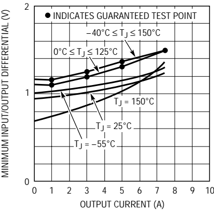
LT1083 Dropout Voltage
