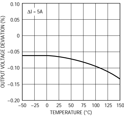
LT1084 Load Regulation
